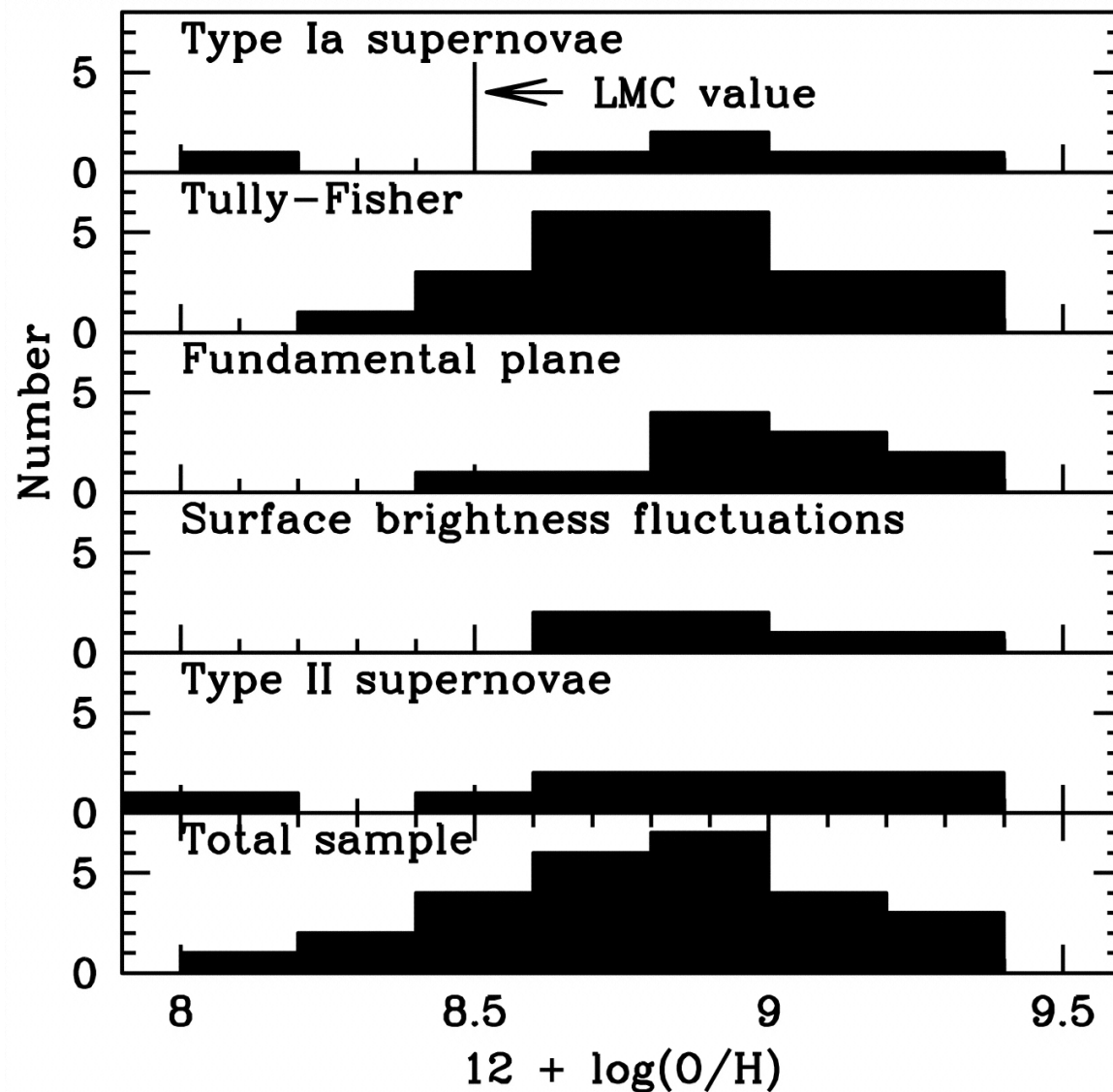
Fig. 6. from Final Results from the Hubble Space Telescope Key Project to Measure the Hubble Constant Freedman et al. 2001 ApJ 553 47 doi:10.1086/320638 https://dx.doi.org/10.1086/320638 © 2001. The American Astronomical Society. All rights reserved. Printed in U.S.A.
