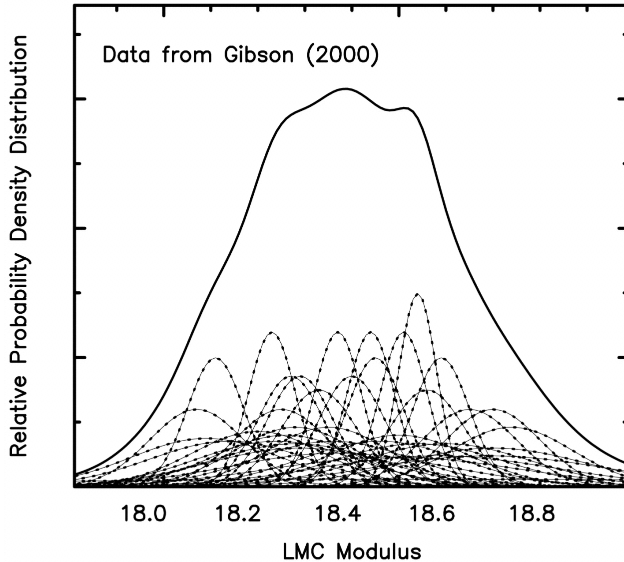
Fig. 5. from Final Results from the Hubble Space Telescope Key Project to Measure the Hubble Constant Freedman et al. 2001 ApJ 553 47 doi:10.1086/320638 https://dx.doi.org/10.1086/320638 © 2001. The American Astronomical Society. All rights reserved. Printed in U.S.A.
