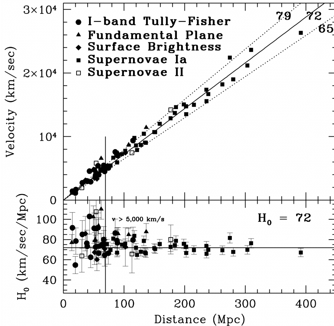
Fig. 4. from Final Results from the Hubble Space Telescope Key Project to Measure the Hubble Constant Freedman et al. 2001 ApJ 553 47 doi:10.1086/320638 https://dx.doi.org/10.1086/320638 © 2001. The American Astronomical Society. All rights reserved. Printed in U.S.A.
