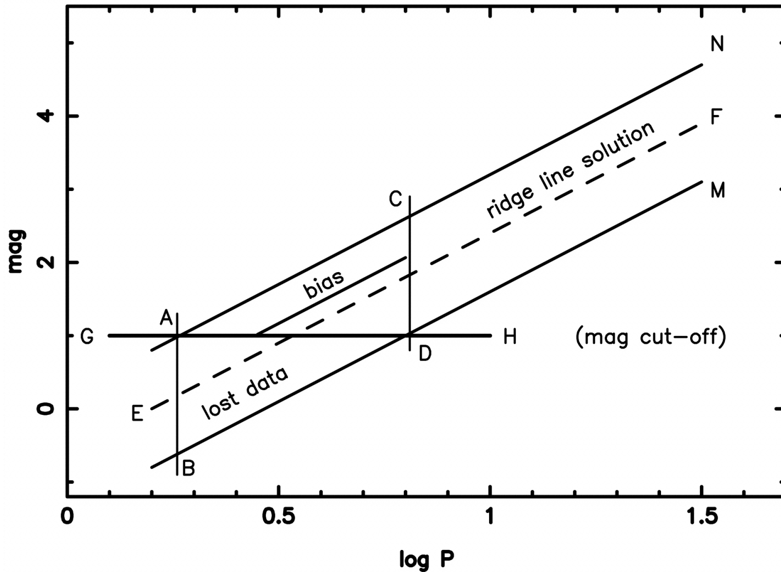
Fig. 10. from Final Results from the Hubble Space Telescope Key Project to Measure the Hubble Constant Freedman et al. 2001 ApJ 553 47 doi:10.1086/320638 https://dx.doi.org/10.1086/320638 © 2001. The American Astronomical Society. All rights reserved. Printed in U.S.A.
