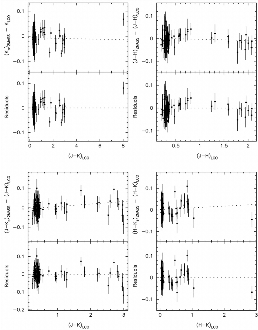
Fig. 9. from Color Transformations for the 2MASS Second Incremental Data Release Carpenter 2001 AJ 121 2851 doi:10.1086/320383 https://dx.doi.org/10.1086/320383 © 2001. The American Astronomical Society. All rights reserved. Printed in U.S.A.
