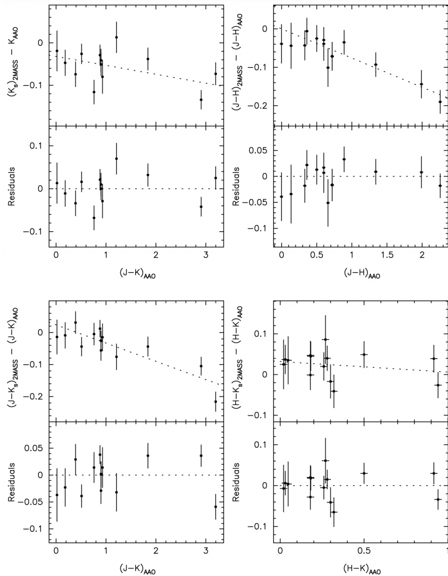
Fig. 4. from Color Transformations for the 2MASS Second Incremental Data Release Carpenter 2001 AJ 121 2851 doi:10.1086/320383 https://dx.doi.org/10.1086/320383 © 2001. The American Astronomical Society. All rights reserved. Printed in U.S.A.
