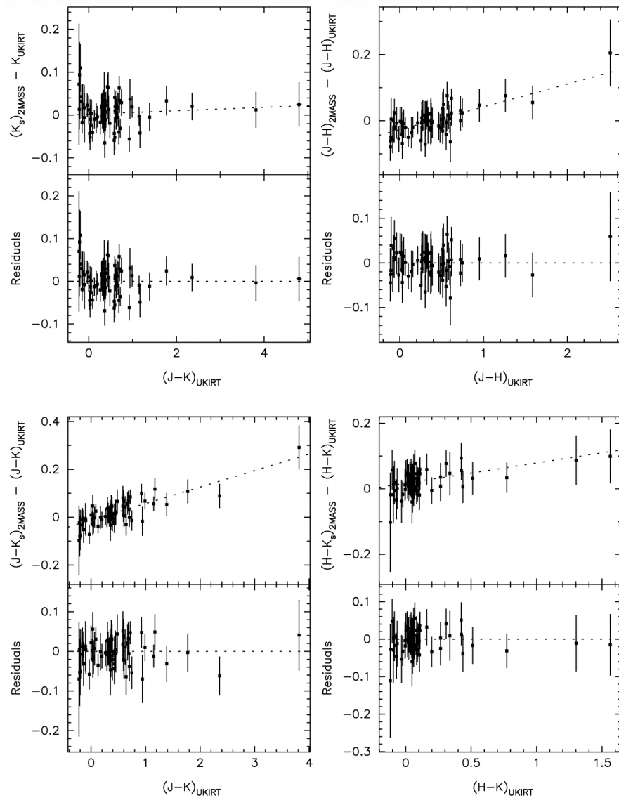
Fig. 13. from Color Transformations for the 2MASS Second Incremental Data Release Carpenter 2001 AJ 121 2851 doi:10.1086/320383 https://dx.doi.org/10.1086/320383 © 2001. The American Astronomical Society. All rights reserved. Printed in U.S.A.
