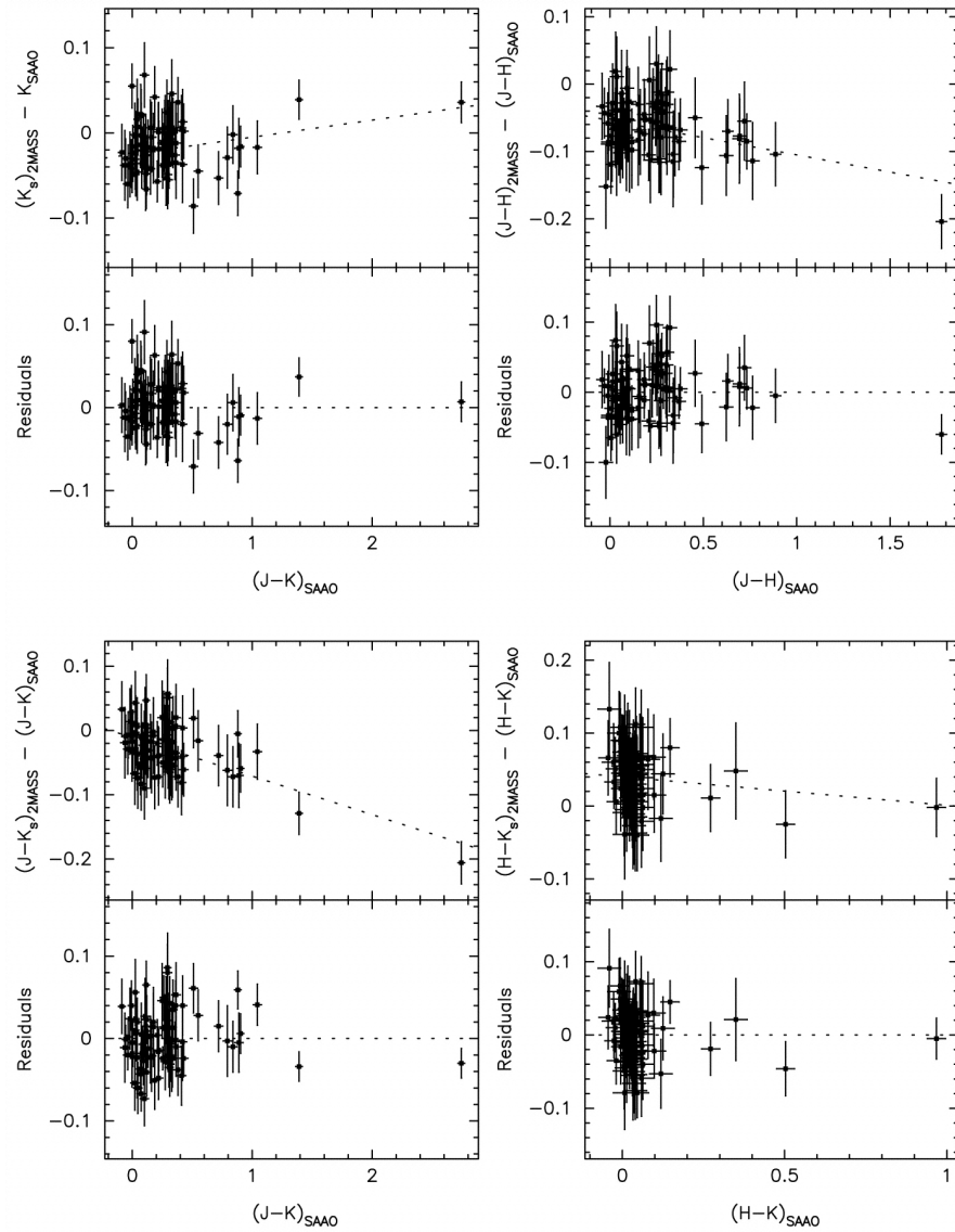
Fig. 12. from Color Transformations for the 2MASS Second Incremental Data Release Carpenter 2001 AJ 121 2851 doi:10.1086/320383 https://dx.doi.org/10.1086/320383 © 2001. The American Astronomical Society. All rights reserved. Printed in U.S.A.
