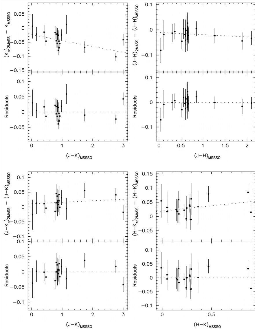
Fig. 11. from Color Transformations for the 2MASS Second Incremental Data Release Carpenter 2001 AJ 121 2851 doi:10.1086/320383 https://dx.doi.org/10.1086/320383 © 2001. The American Astronomical Society. All rights reserved. Printed in U.S.A.
