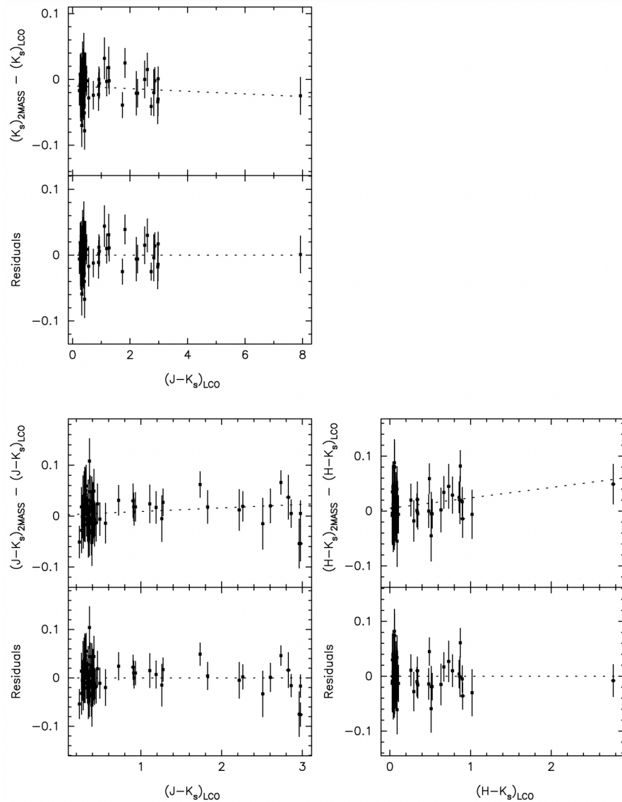
Fig. 10. from Color Transformations for the 2MASS Second Incremental Data Release Carpenter 2001 AJ 121 2851 doi:10.1086/320383 https://dx.doi.org/10.1086/320383 © 2001. The American Astronomical Society. All rights reserved. Printed in U.S.A.
