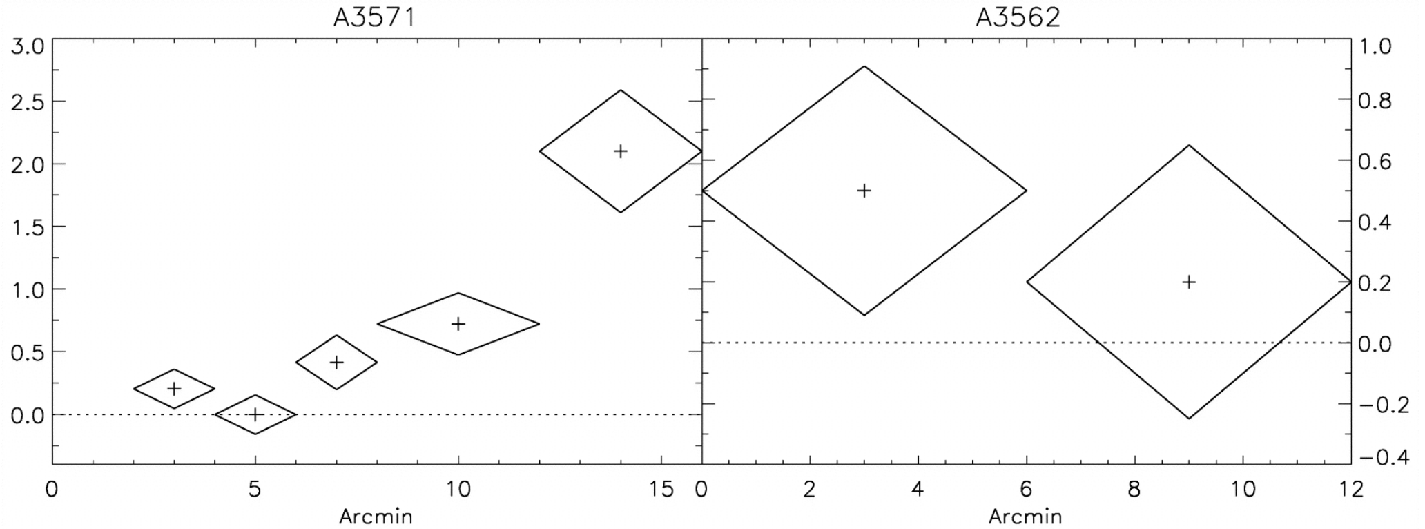
Fig. 4. from ROSAT and BeppoSAX Evidence of Soft XRay Excess Emission in the Shapley Supercluster: A3571, A3558, A3560, and A3562 Bonamente et al. 2001 ApJL 552 L7 doi:10.1086/320259 https://dx.doi.org/10.1086/320259 © 2001. The American Astronomical Society. All rights reserved. Printed in U.S.A.
