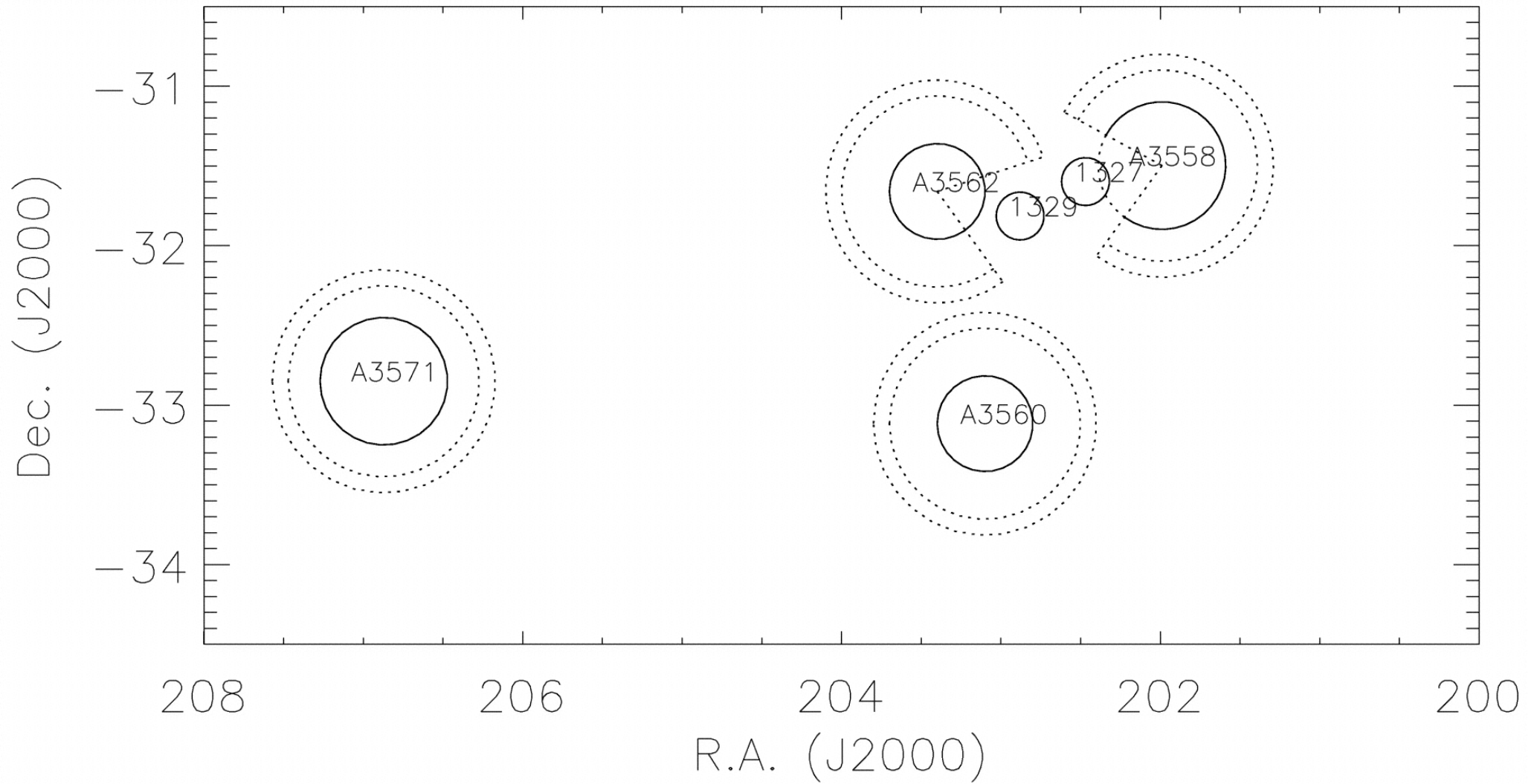
Fig. 1. from ROSAT and BeppoSAX Evidence of Soft XRay Excess Emission in the Shapley Supercluster: A3571, A3558, A3560, and A3562 Bonamente et al. 2001 ApJL 552 L7 doi:10.1086/320259 https://dx.doi.org/10.1086/320259 © 2001. The American Astronomical Society. All rights reserved. Printed in U.S.A.
