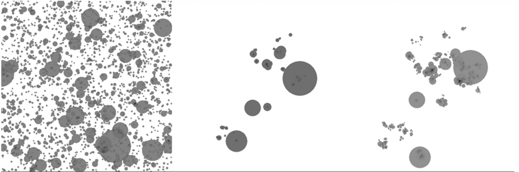
Fig. 3. from Fractal Structure in Galactic Star Fields Elmegreen & Elmegreen 2001 AJ 121 1507 doi:10.1086/319416 https://dx.doi.org/10.1086/319416 © 2001. The American Astronomical Society. All rights reserved. Printed in U.S.A.
