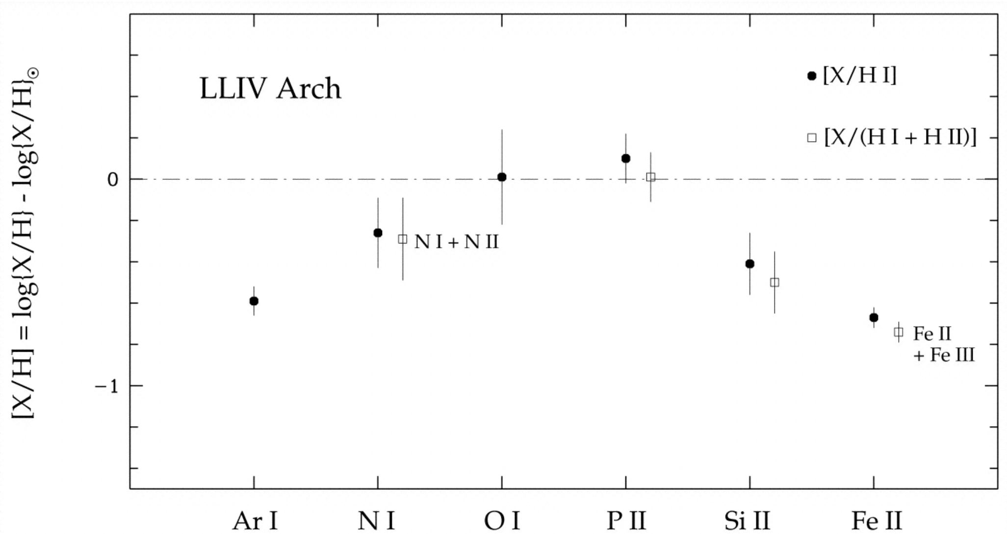
Fig. 5. from The FUSE Spectrum of PG 0804+761: A Study of Atomic and Molecular Gas in the Lower Galactic Halo and Beyond Richter et al. 2001 ApJ 549 281 doi:10.1086/319070 https://dx.doi.org/10.1086/319070 © 2001. The American Astronomical Society. All rights reserved. Printed in U.S.A.
