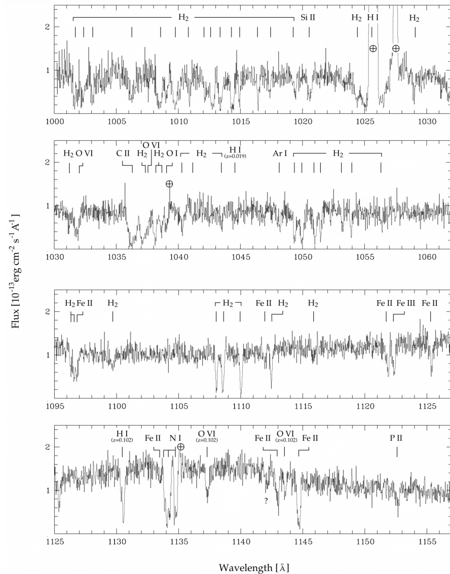
Fig. 2. from The FUSE Spectrum of PG 0804+761: A Study of Atomic and Molecular Gas in the Lower Galactic Halo and Beyond Richter et al. 2001 ApJ 549 281 doi:10.1086/319070 https://dx.doi.org/10.1086/319070 © 2001. The American Astronomical Society. All rights reserved. Printed in U.S.A.
