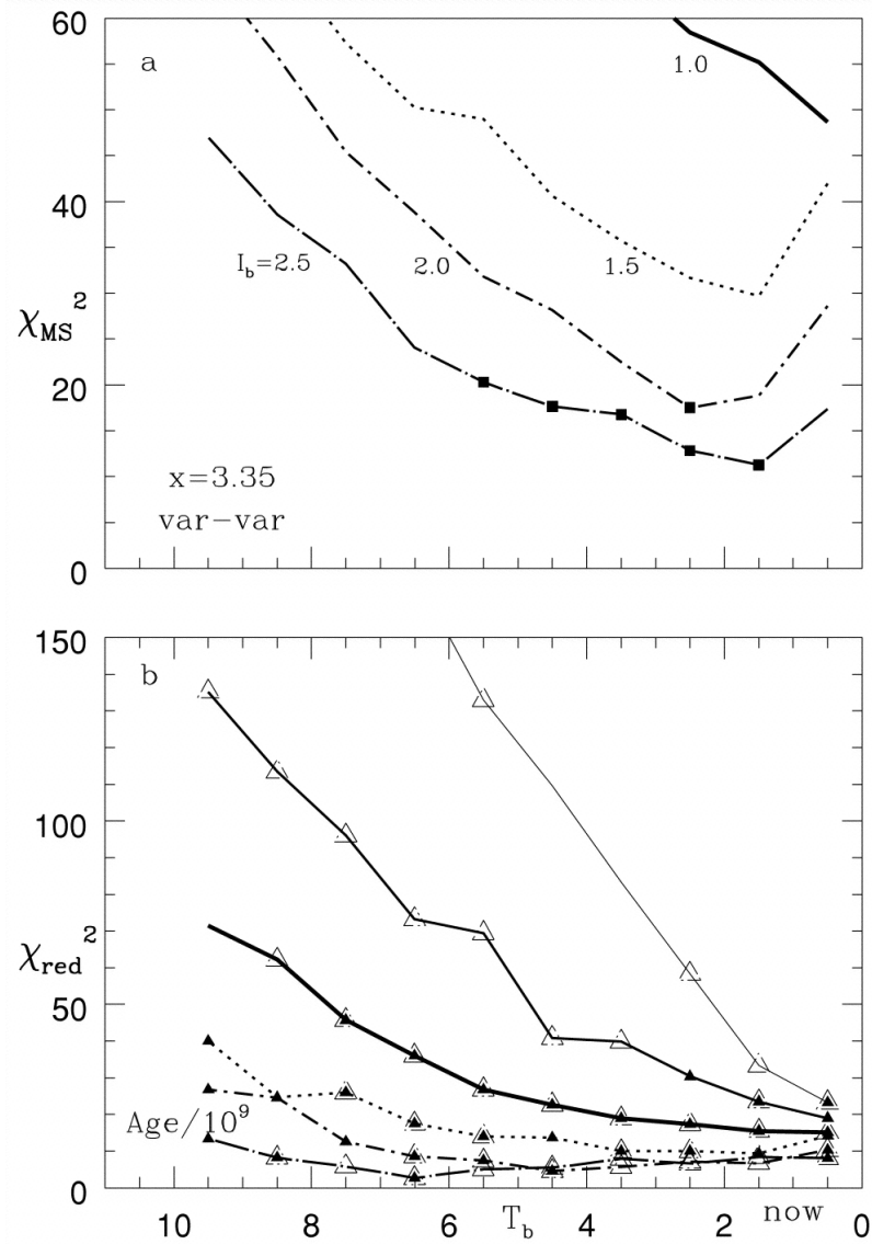
Fig. 7. from Star Formation History in the Solar Vicinity Bertelli & Nasi 2001 AJ 121 1013 doi:10.1086/318781 https://dx.doi.org/10.1086/318781 © 2001. The American Astronomical Society. All rights reserved. Printed in U.S.A.
