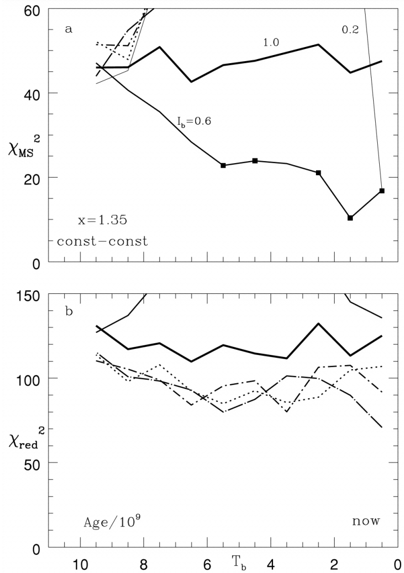
Fig. 6. from Star Formation History in the Solar Vicinity Bertelli & Nasi 2001 AJ 121 1013 doi:10.1086/318781 https://dx.doi.org/10.1086/318781 © 2001. The American Astronomical Society. All rights reserved. Printed in U.S.A.
