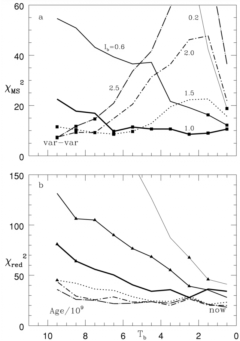
Fig. 5. from Star Formation History in the Solar Vicinity Bertelli & Nasi 2001 AJ 121 1013 doi:10.1086/318781 https://dx.doi.org/10.1086/318781 © 2001. The American Astronomical Society. All rights reserved. Printed in U.S.A.
