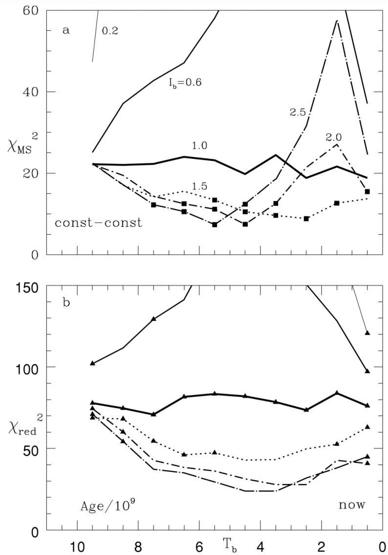
Fig. 4. from Star Formation History in the Solar Vicinity Bertelli & Nasi 2001 AJ 121 1013 doi:10.1086/318781 https://dx.doi.org/10.1086/318781 © 2001. The American Astronomical Society. All rights reserved. Printed in U.S.A.
