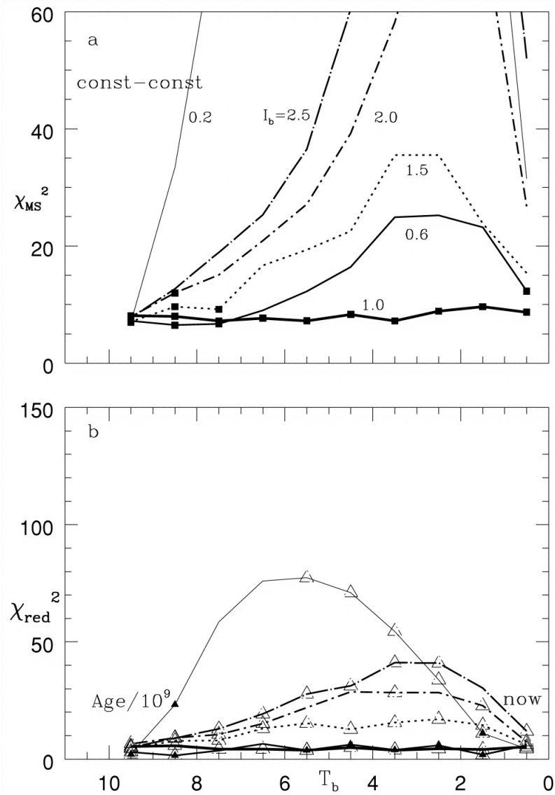
Fig. 3. from Star Formation History in the Solar Vicinity Bertelli & Nasi 2001 AJ 121 1013 doi:10.1086/318781 https://dx.doi.org/10.1086/318781 © 2001. The American Astronomical Society. All rights reserved. Printed in U.S.A.
