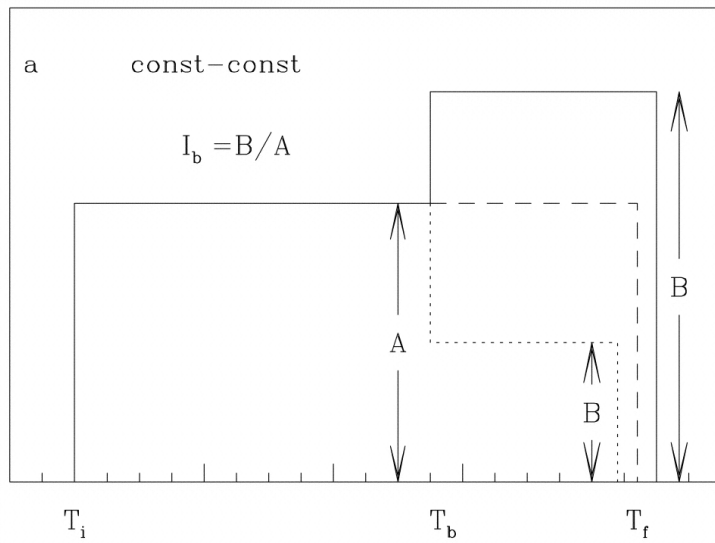
Fig. 2. from Star Formation History in the Solar Vicinity Bertelli & Nasi 2001 AJ 121 1013 doi:10.1086/318781 https://dx.doi.org/10.1086/318781 © 2001. The American Astronomical Society. All rights reserved. Printed in U.S.A.
