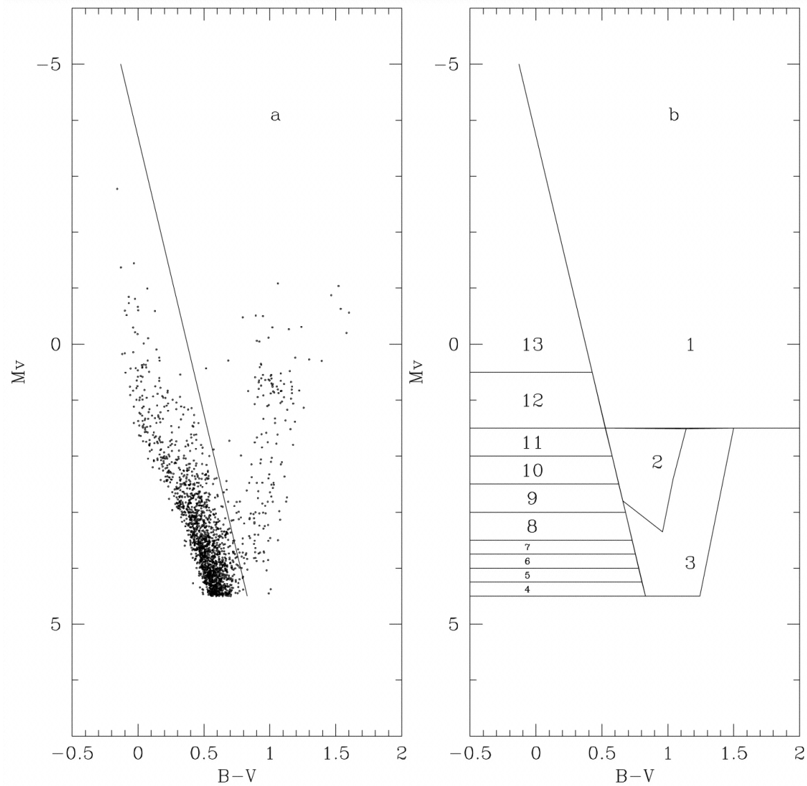
Fig. 1. from Star Formation History in the Solar Vicinity Bertelli & Nasi 2001 AJ 121 1013 doi:10.1086/318781 https://dx.doi.org/10.1086/318781 © 2001. The American Astronomical Society. All rights reserved. Printed in U.S.A.
