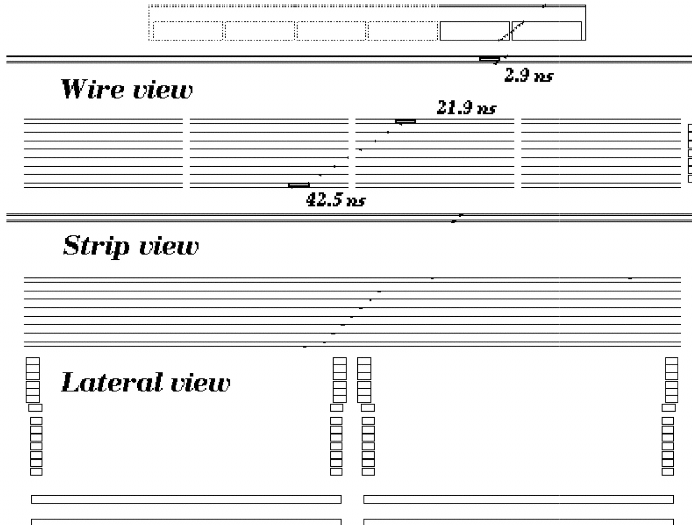
Fig. 3. from Neutrino Astronomy with the MACRO Detector Ambrosio et al. 2001 ApJ 546 1038 doi:10.1086/318281 https://dx.doi.org/10.1086/318281 © 2001. The American Astronomical Society. All rights reserved. Printed in U.S.A.
