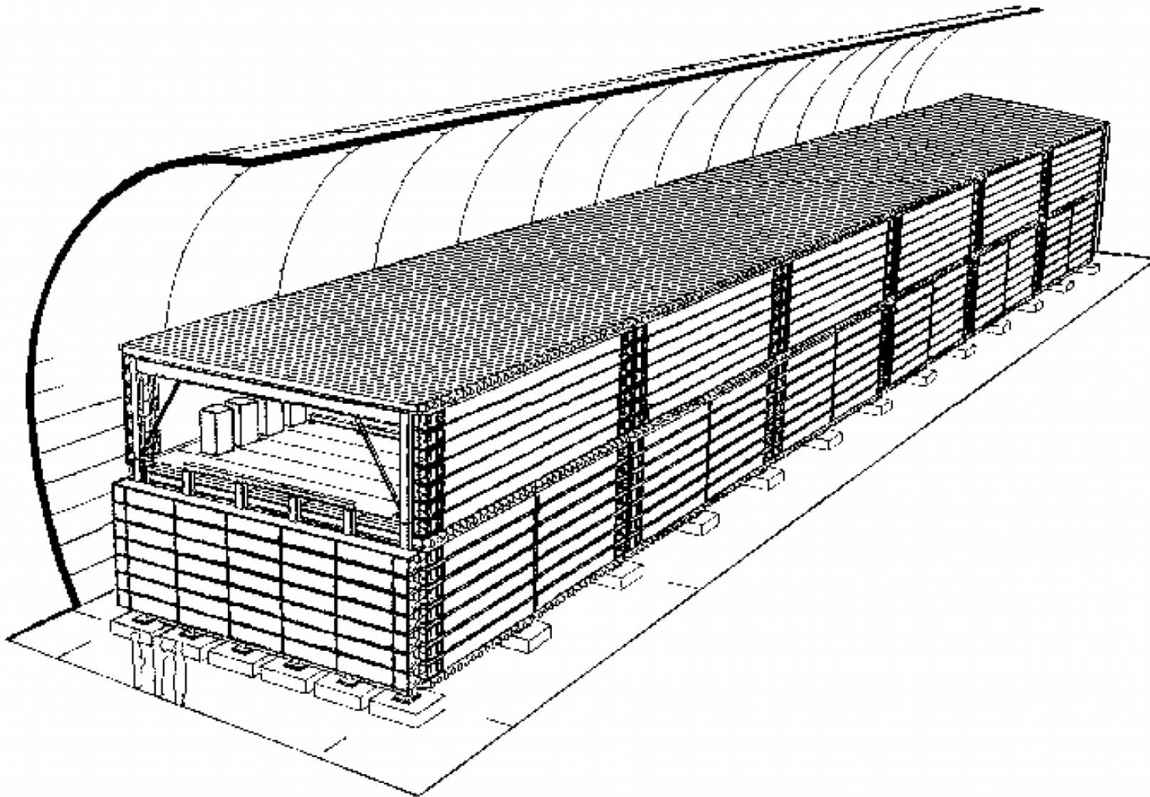
Fig. 1. from Neutrino Astronomy with the MACRO Detector Ambrosio et al. 2001 ApJ 546 1038 doi:10.1086/318281 https://dx.doi.org/10.1086/318281 © 2001. The American Astronomical Society. All rights reserved. Printed in U.S.A.
