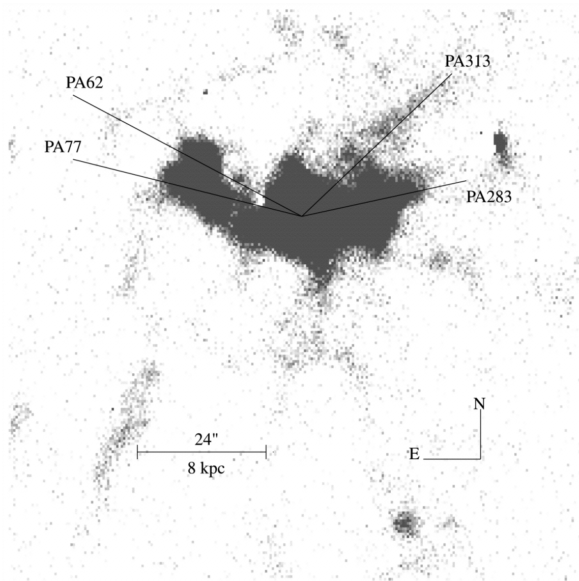
Fig. 1. from EmissionLine Properties of the Optical Filaments of NGC 1275 Sabra, Shields, & Filippenko 2000 ApJ 545 157 doi:10.1086/317793 https://dx.doi.org/10.1086/317793 © 2000. The American Astronomical Society. All rights reserved. Printed in U.S.A.
