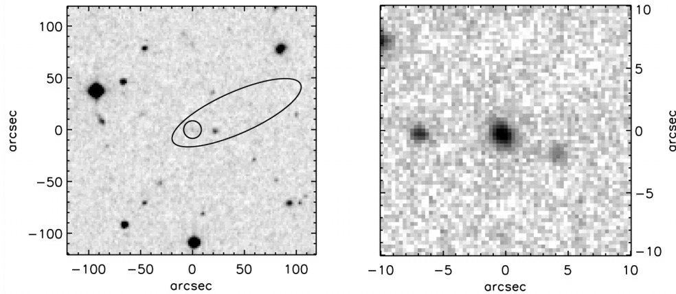
FF1032+3453, z=0.255
