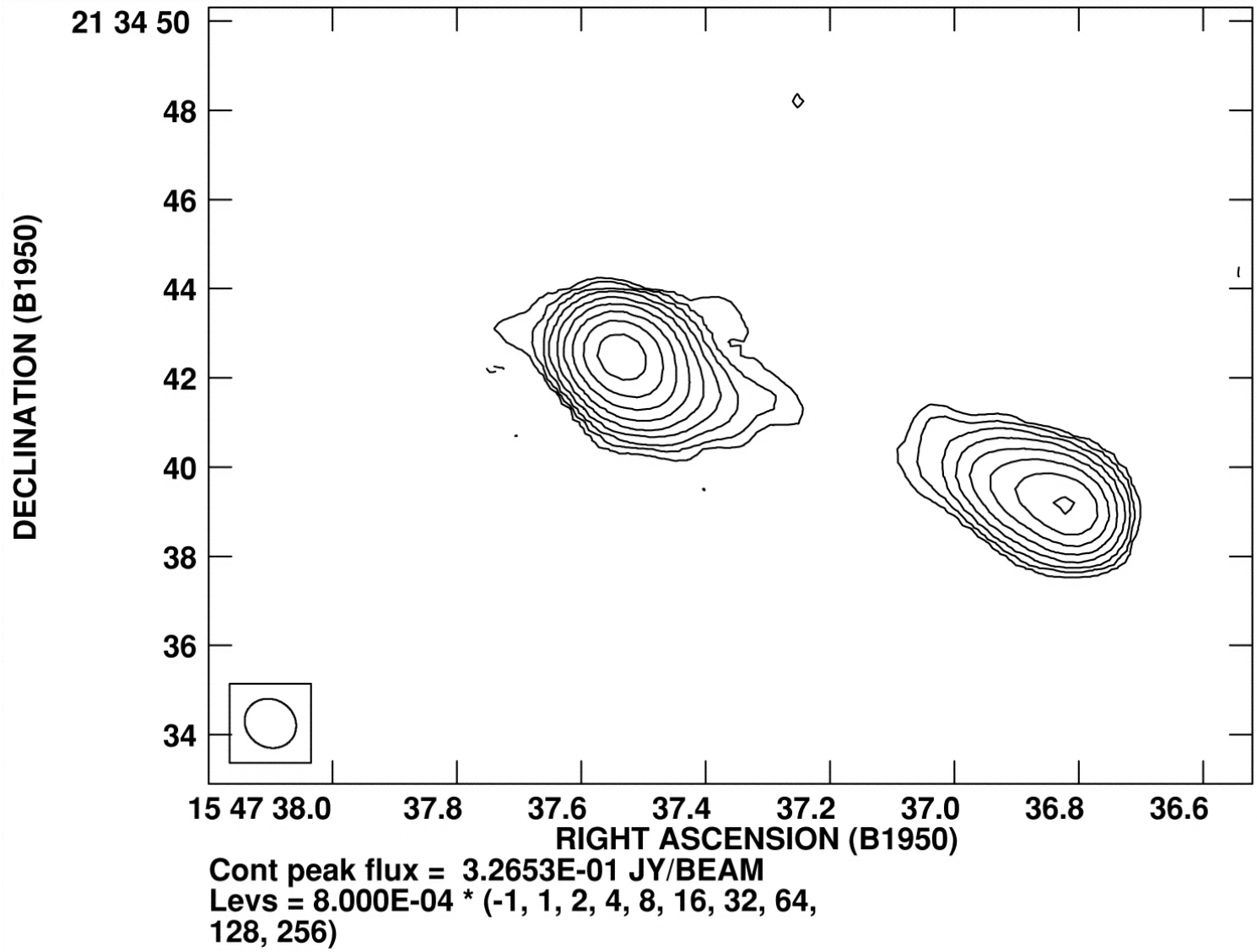
Fig. 5. from Global Cosmological Parameters Determined Using Classical Double Radio Galaxies Guerra, Daly, & Wan 2000 ApJ 544 659 doi:10.1086/317217 https://dx.doi.org/10.1086/317217 © 2000. The American Astronomical Society. All rights reserved. Printed in U.S.A.
