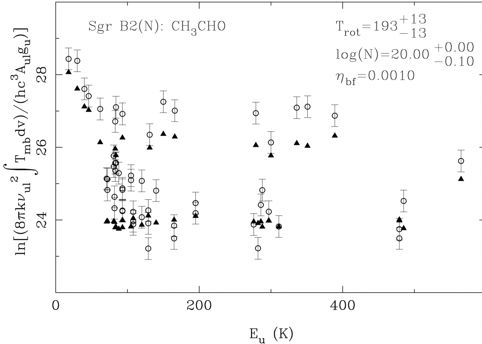
Fig. 4. from A ThreePosition Spectral Line Survey of Sagittarius B2 between 218 and 263 GHz. II. Data Analysis Nummelin et al. 2000 ApJS 128 213 doi:10.1086/313376 https://dx.doi.org/10.1086/313376 © 2000. The American Astronomical Society. All rights reserved. Printed in U.S.A.
