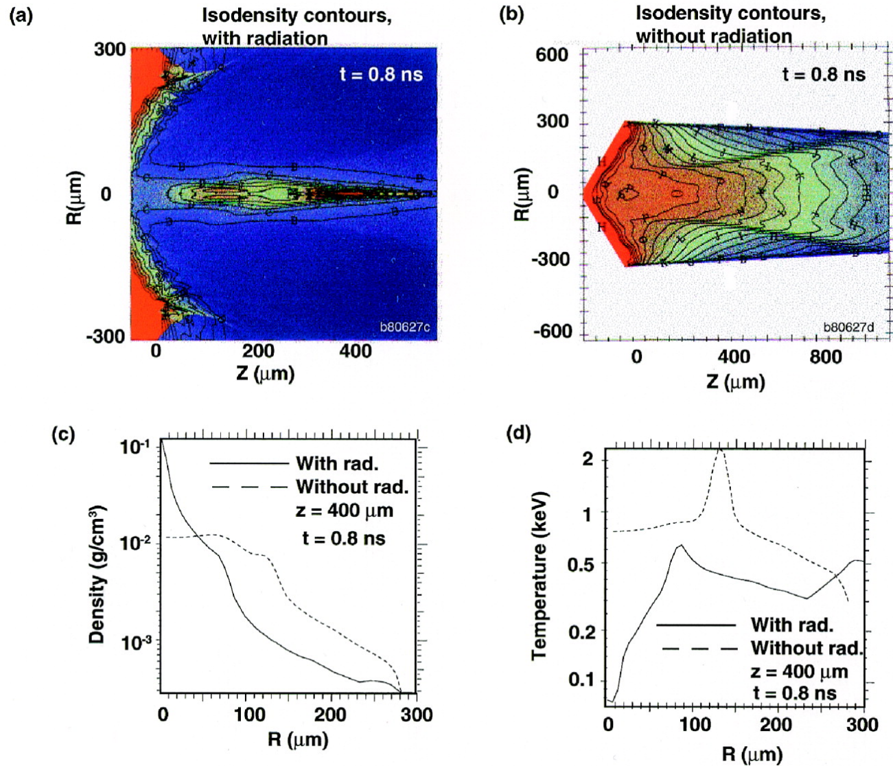
Fig. 5. from Testing Astrophysical Radiation Hydrodynamics Codes with Hypervelocity Jet Experiments on the Nova Laser Stone et al. 2000 ApJS 127 497 doi:10.1086/313337 https://dx.doi.org/10.1086/313337 © 2000. The American Astronomical Society. All rights reserved. Printed in U.S.A.
