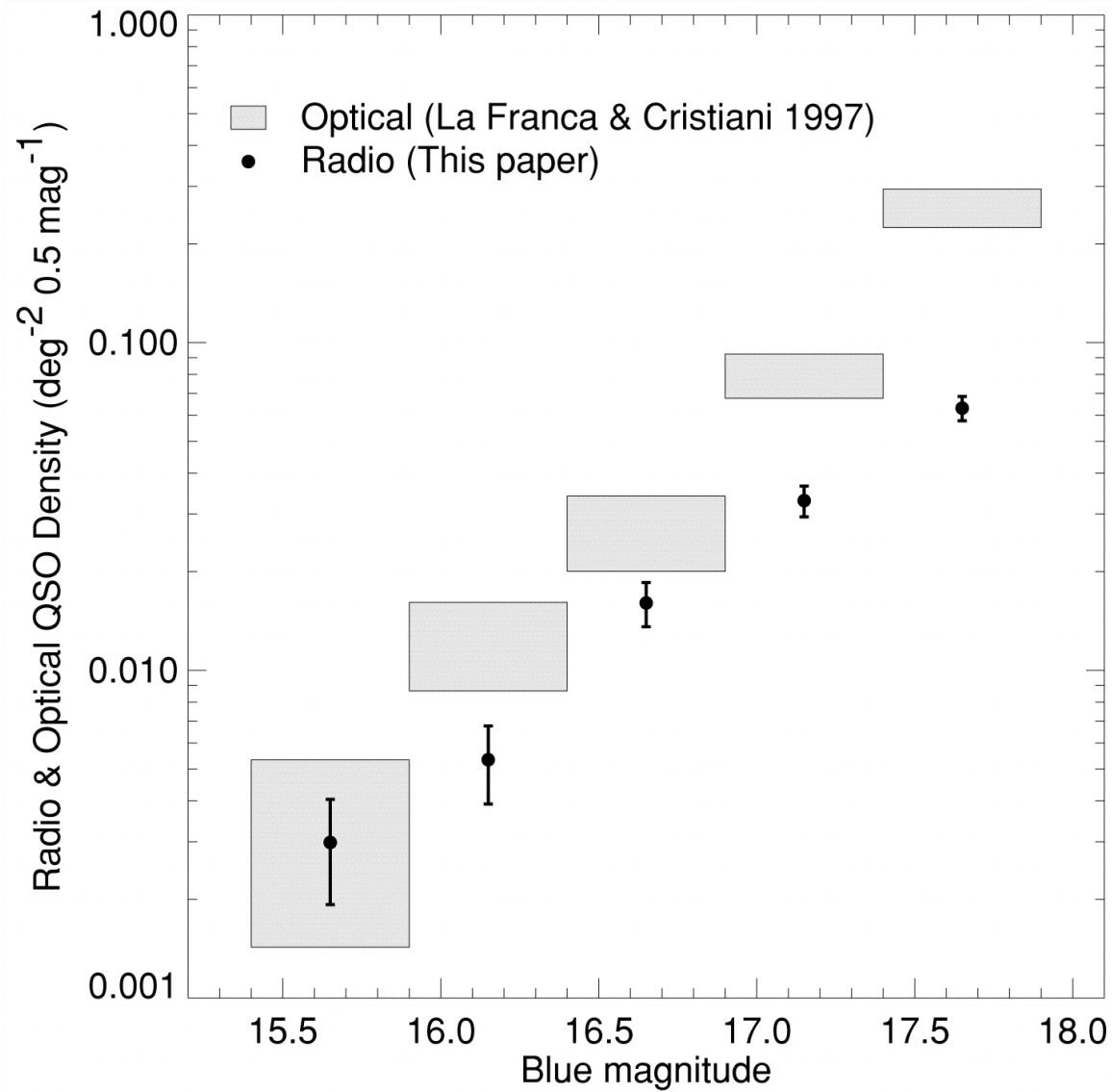
Fig. 13. from The FIRST Bright Quasar Survey. II. 60 Nights and 1200 Spectra Later White et al. 2000 ApJS 126 133 doi:10.1086/313300 https://dx.doi.org/10.1086/313300 © 2000. The American Astronomical Society. All rights reserved. Printed in U.S.A.
