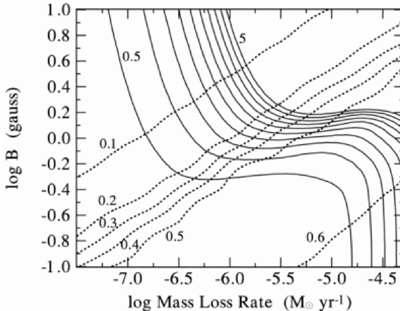
Fig. 9. from XRay and Radio Observations of the Cygnus OB2 Association Waldron et al. 1998 ApJS 118 217 doi:10.1086/313131 https://dx.doi.org/10.1086/313131 ©1998. The American Astronomical Society. All rights reserved. Printed in U.S.A.
