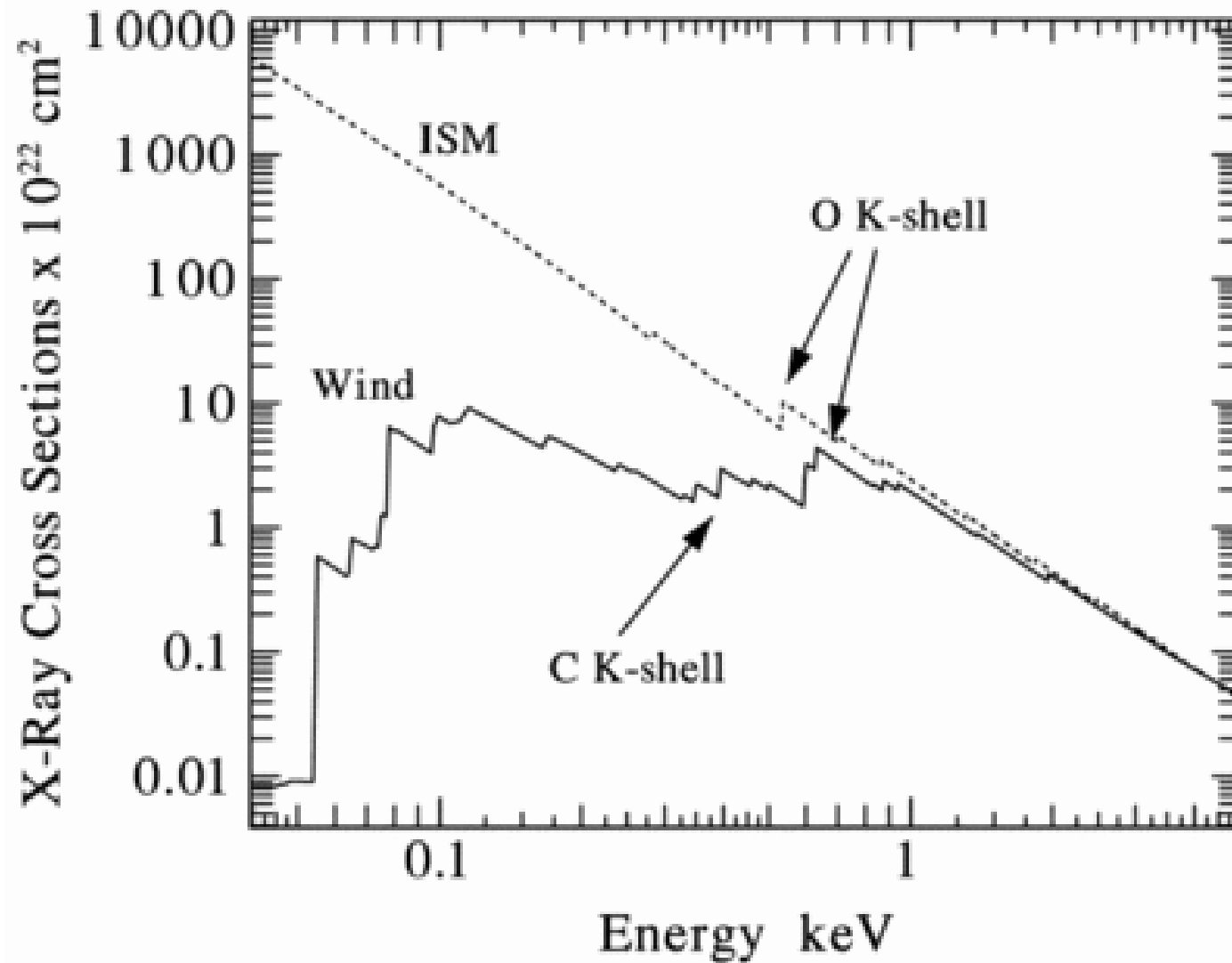
Fig. 2. from XRay and Radio Observations of the Cygnus OB2 Association Waldron et al. 1998 ApJS 118 217 doi:10.1086/313131 https://dx.doi.org/10.1086/313131 ©1998. The American Astronomical Society. All rights reserved. Printed in U.S.A.
