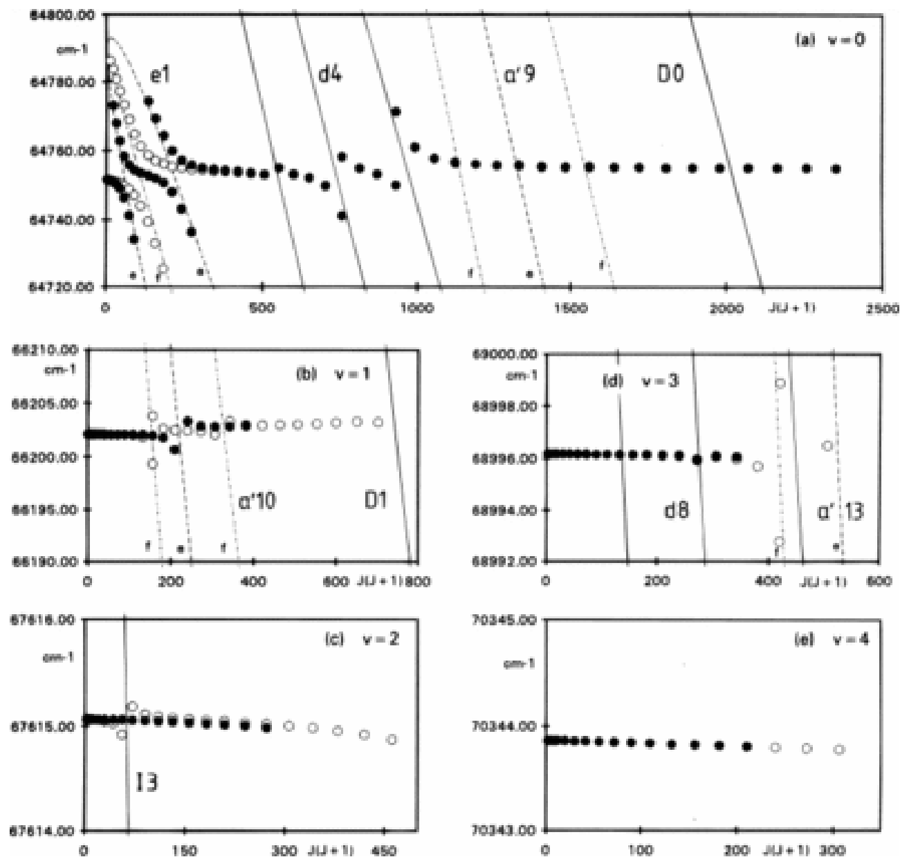
Fig. 2. from A HighResolution ^{18}\text{O} Isotope Study in the Vacuum Ultraviolet of the A\ 1\ X\ 1+ 4\text{th Positive System of CO} Beaty et al. 1997 ApJS 109 269 doi:10.1086/312976 https://dx.doi.org/10.1086/312976
