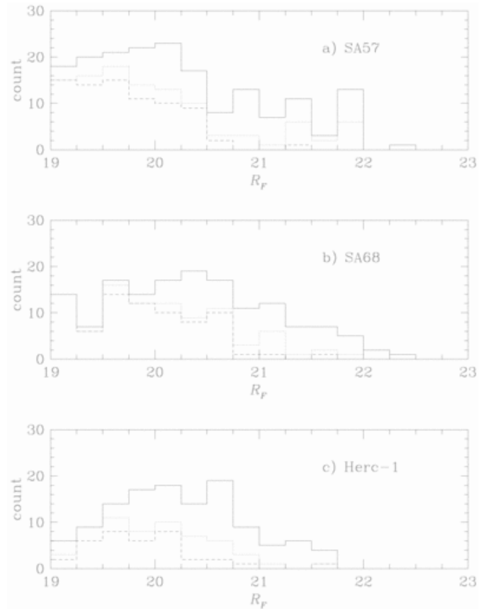
Fig. 4. from The Kitt Peak Galaxy Redshift Survey with Multicolor Photometry: Basic Data Munn et al. 1997 ApJS 109 45 doi:10.1086/312971 https://dx.doi.org/10.1086/312971
