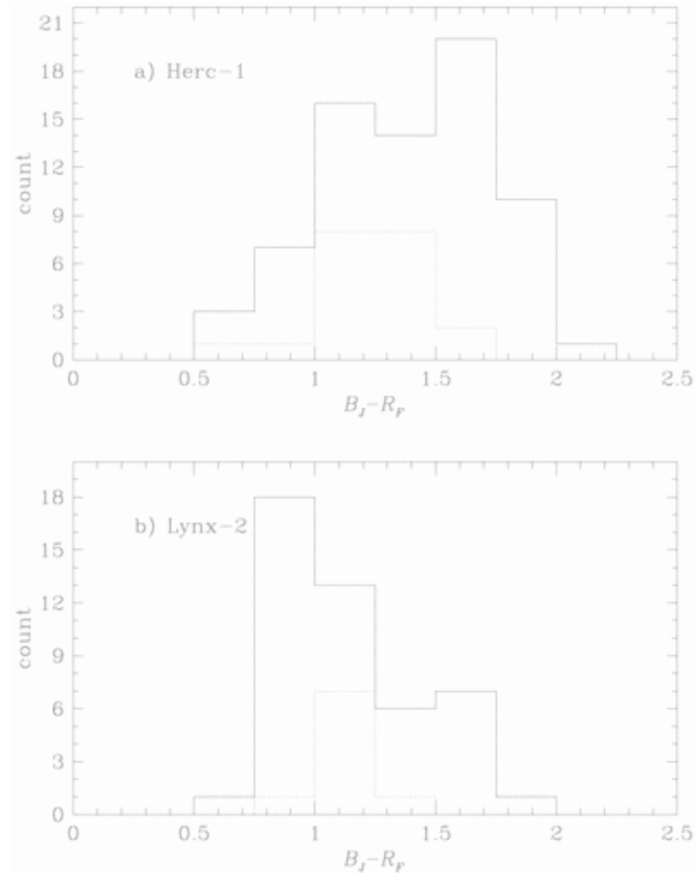
Fig. 3. from The Kitt Peak Galaxy Redshift Survey with Multicolor Photometry: Basic Data Munn et al. 1997 ApJS 109 45 doi:10.1086/312971 https://dx.doi.org/10.1086/312971 © 1997. The American Astronomical Society. All rights reserved. Printed in U.S.A.
