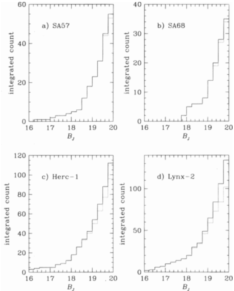
Fig. 2. from The Kitt Peak Galaxy Redshift Survey with Multicolor Photometry: Basic Data Munn et al. 1997 ApJS 109 45 doi:10.1086/312971 https://dx.doi.org/10.1086/312971
