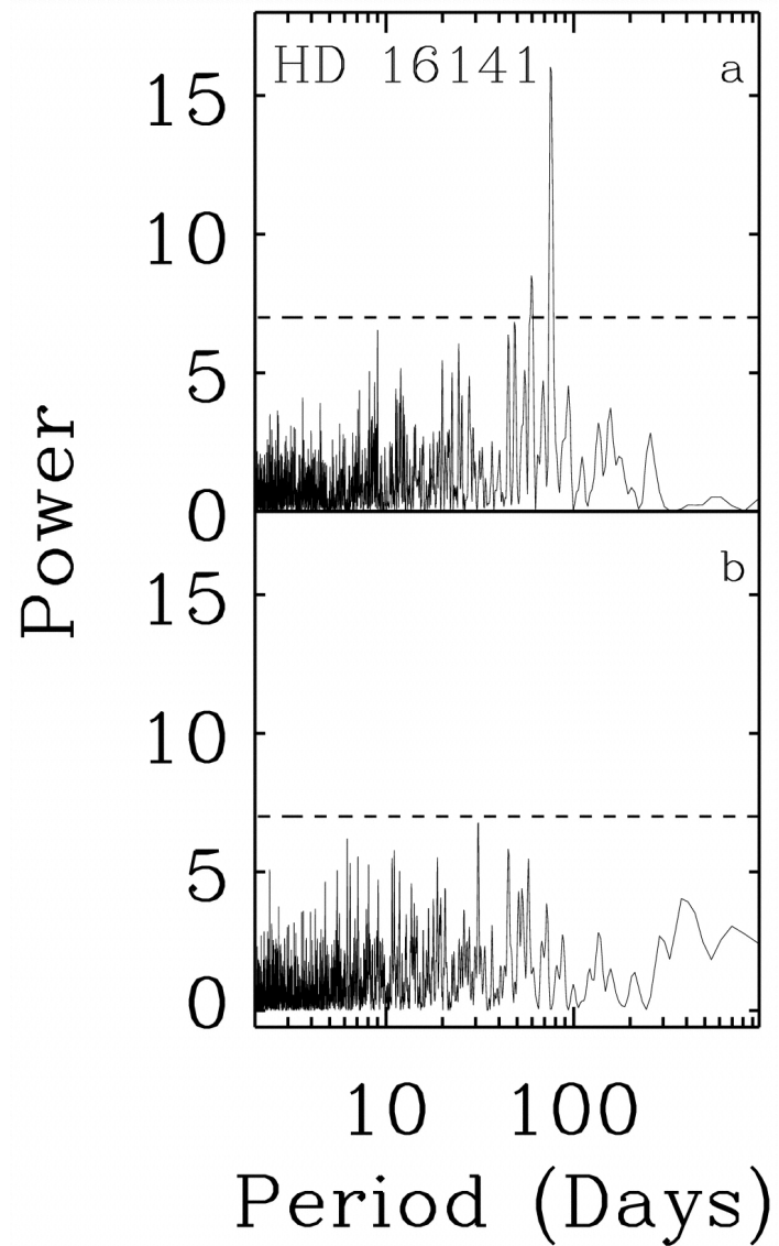
Fig. 2. from SubSaturn Planetary Candidates of HD 16141 and HD 46375 Marcy, Butler, & Vogt 2000 ApJL 536 L43 doi:10.1086/312723 https://dx.doi.org/10.1086/312723 © 2000. The American Astronomical Society. All rights reserved. Printed in U.S.A.
