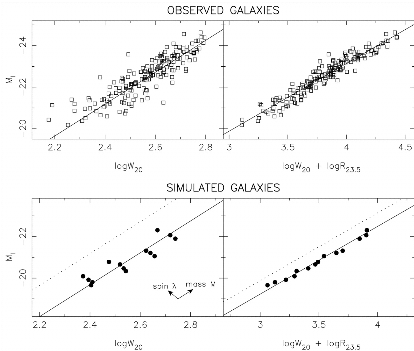
Fig. 2. from A Unified Scaling Law in Spiral Galaxies Koda, Sofue, & Wada 2000 ApJL 531 L17 doi:10.1086/312509 https://dx.doi.org/10.1086/312509 © 2000. The American Astronomical Society. All rights reserved. Printed in U.S.A.
