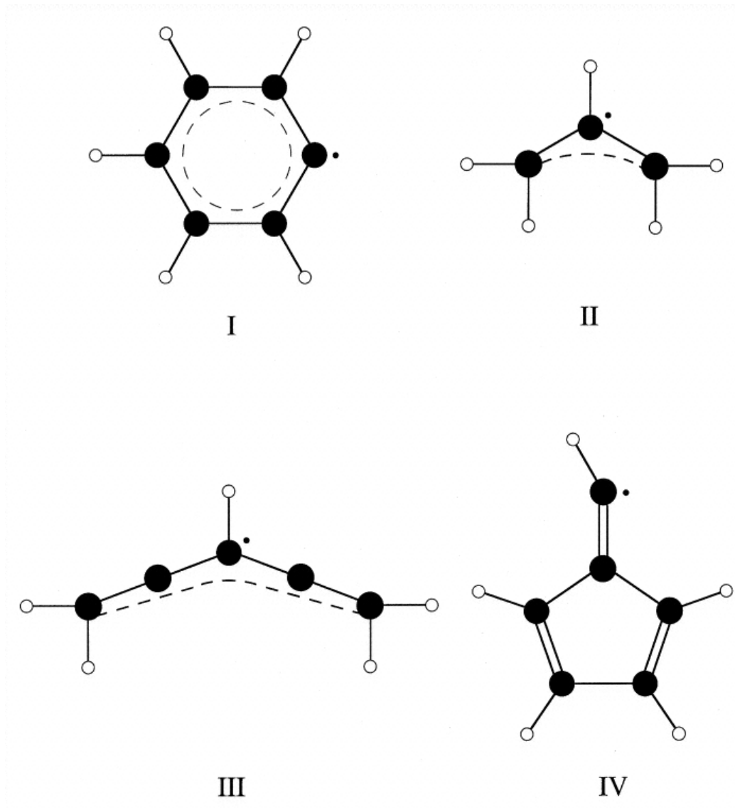
Fig. 3. from Laboratory Detection of a Molecular Band at 4429 Ball, McCarthy, & Thaddeus 2000 ApJL 529 L61 doi:10.1086/312449 https://dx.doi.org/10.1086/312449 © 2000. The American Astronomical Society. All rights reserved. Printed in U.S.A.
