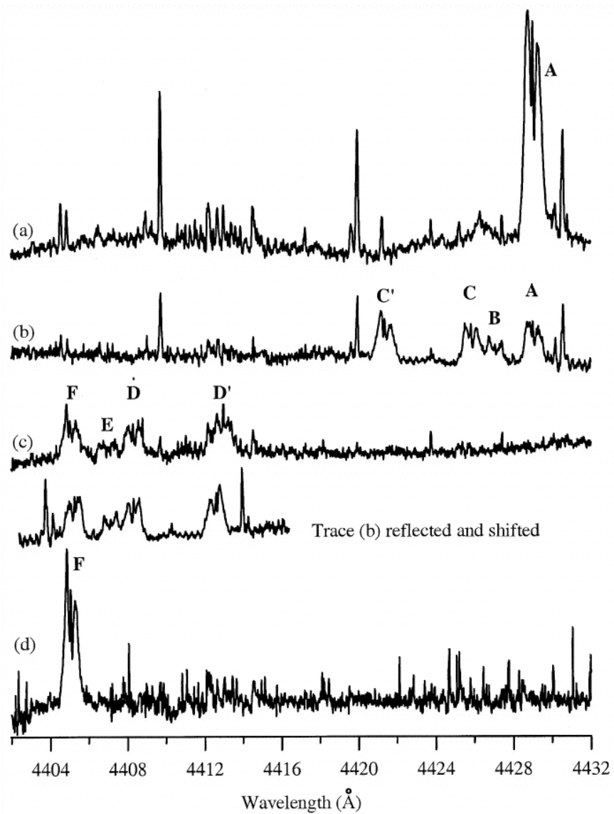
Fig. 2. from Laboratory Detection of a Molecular Band at 4429 Ball, McCarthy, & Thaddeus 2000 ApJL 529 L61 doi:10.1086/312449 https://dx.doi.org/10.1086/312449 © 2000. The American Astronomical Society. All rights reserved. Printed in U.S.A.
