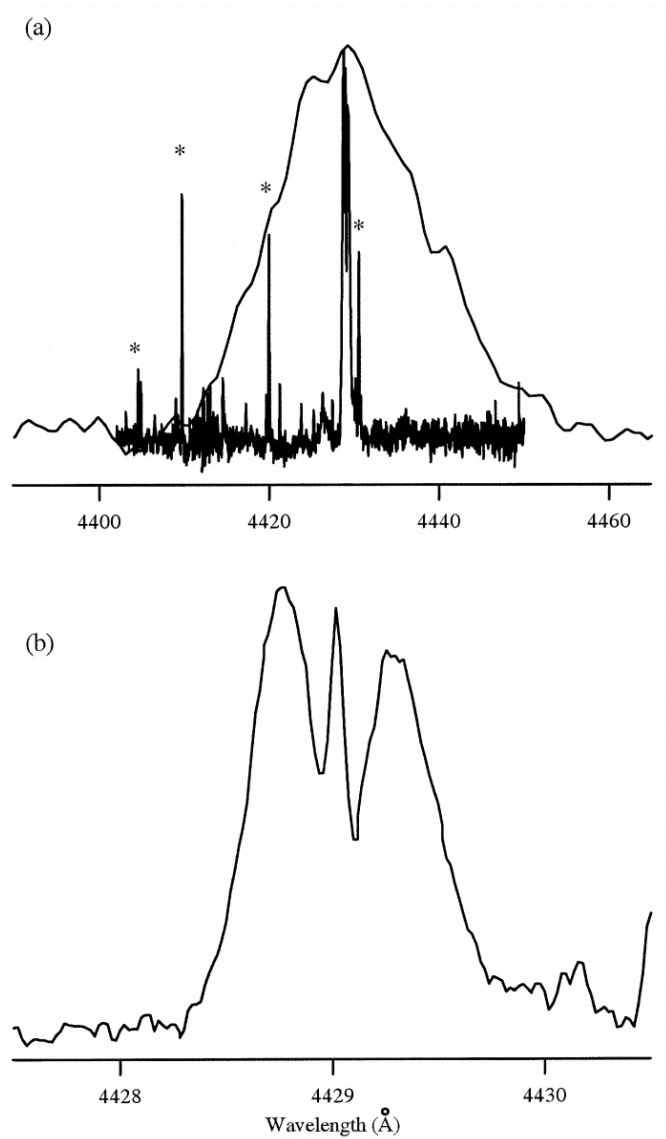
Fig. 1. from Laboratory Detection of a Molecular Band at 4429 Ball, McCarthy, & Thaddeus 2000 ApJL 529 L61 doi:10.1086/312449 https://dx.doi.org/10.1086/312449 © 2000. The American Astronomical Society. All rights reserved. Printed in U.S.A.
