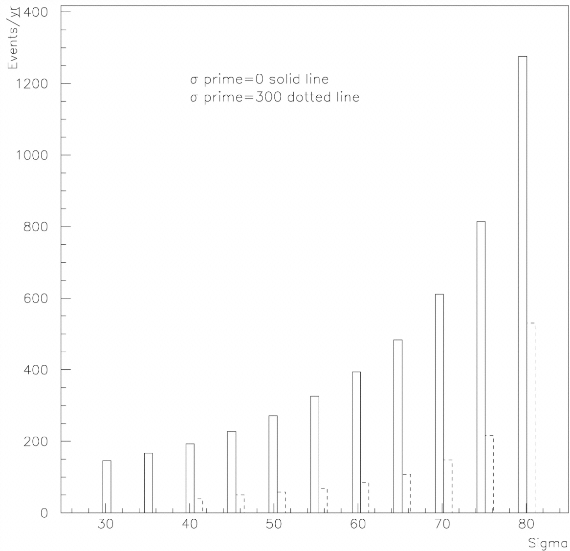
Fig. 1. from Neutrino Event Rates from GammaRay Bursts Halzen & Hooper 1999 ApJL 527 L93 doi:10.1086/312403 https://dx.doi.org/10.1086/312403 © 1999. The American Astronomical Society. All rights reserved. Printed in U.S.A.
