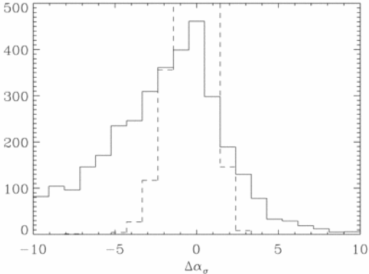
Fig. 3. from The Synchrotron Shock Model Confronts a “Line of Death” in the BATSE GammaRay Burst Data Preece et al. 1998 ApJL 506 L23 doi:10.1086/311644 https://dx.doi.org/10.1086/311644 © 1998. The American Astronomical Society. All rights reserved. Printed in U.S.A.
