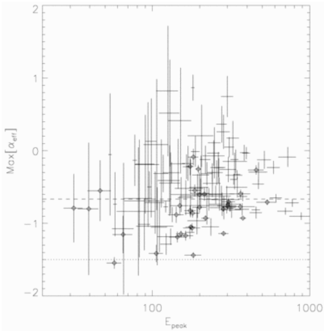
Fig. 2. from The Synchrotron Shock Model Confronts a “Line of Death” in the BATSE GammaRay Burst Data Preece et al. 1998 ApJL 506 L23 doi:10.1086/311644 https://dx.doi.org/10.1086/311644 © 1998. The American Astronomical Society. All rights reserved. Printed in U.S.A.
