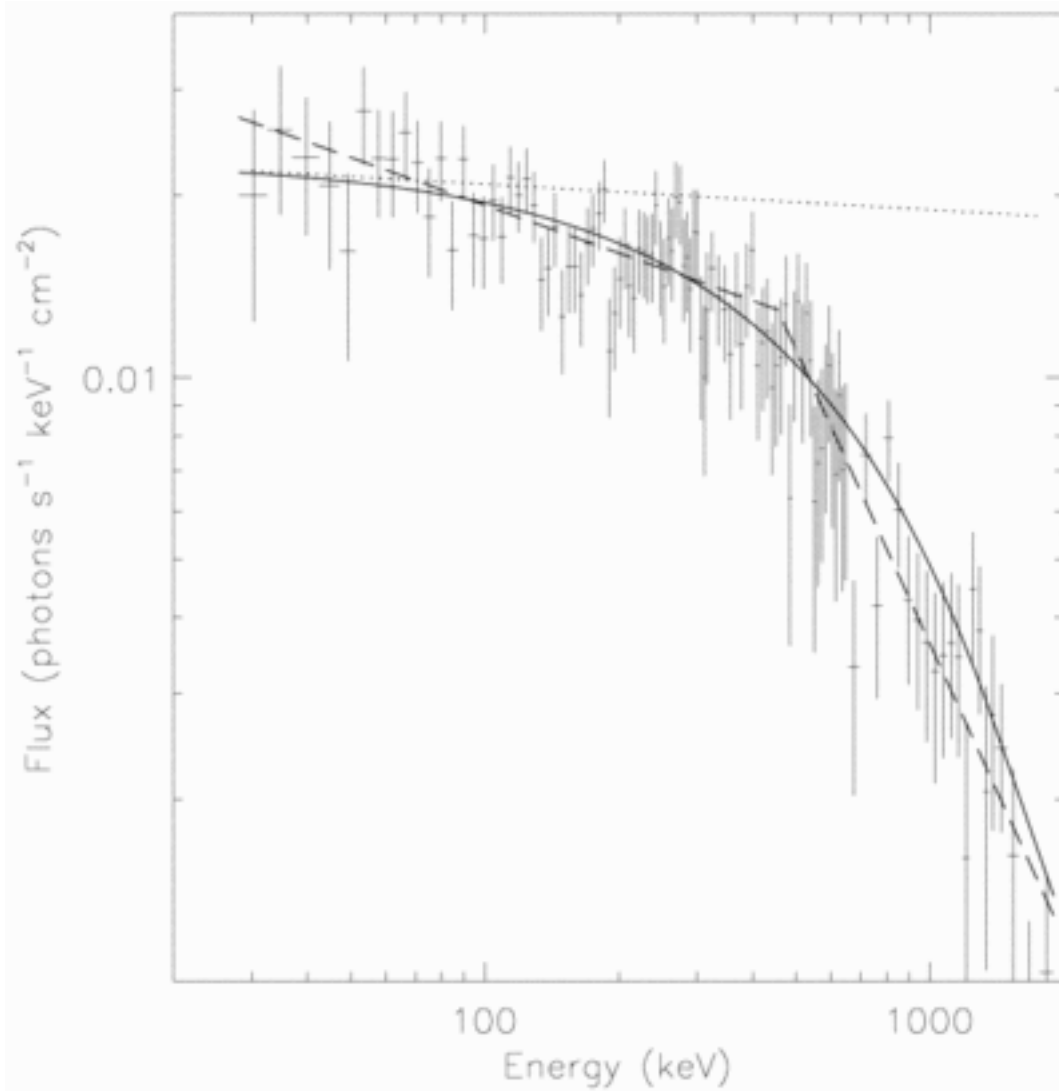
Fig. 1. from The Synchrotron Shock Model Confronts a “Line of Death” in the BATSE GammaRay Burst Data Preece et al. 1998 ApJL 506 L23 doi:10.1086/311644 https://dx.doi.org/10.1086/311644 © 1998. The American Astronomical Society. All rights reserved. Printed in U.S.A.
