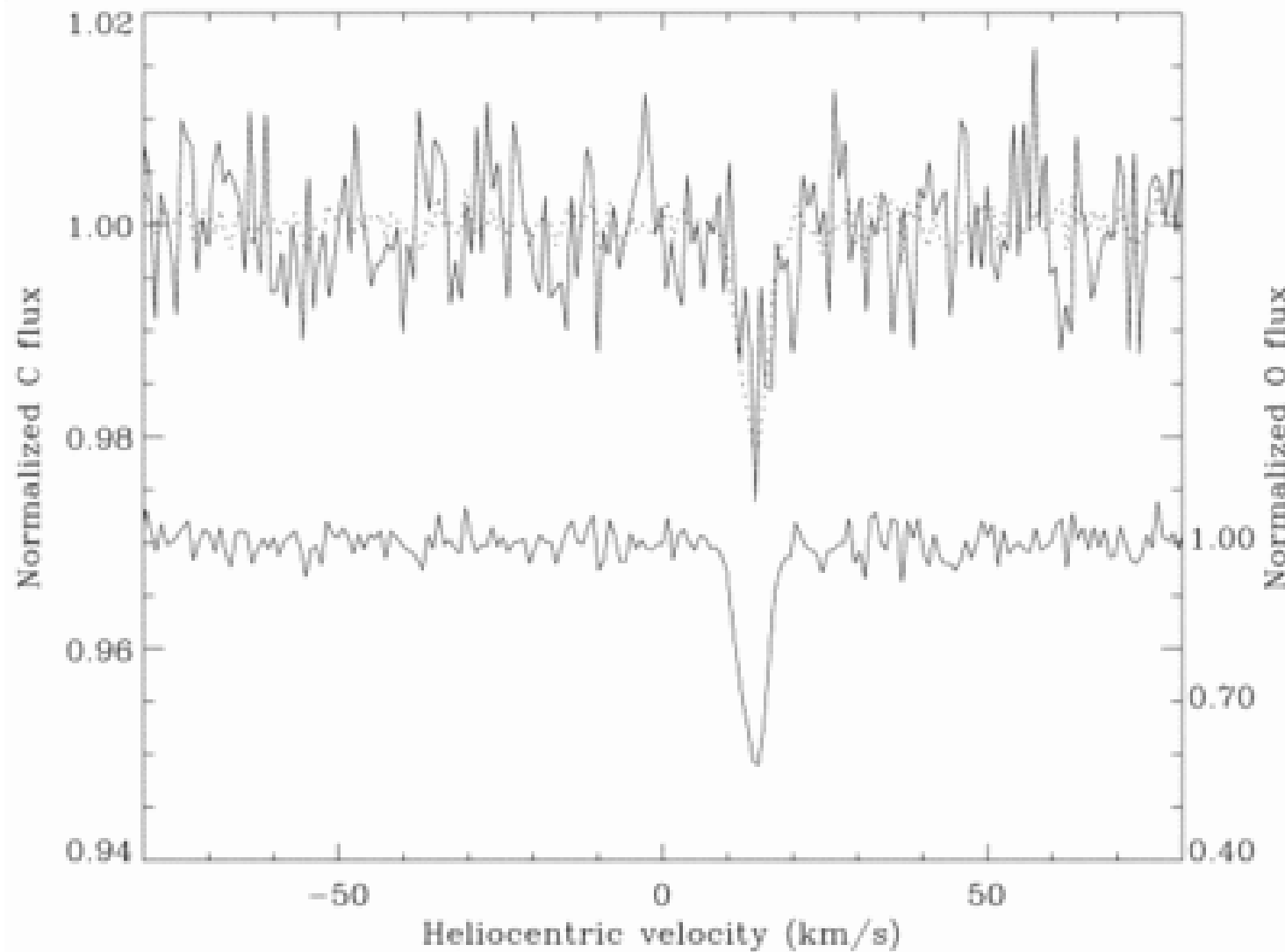
Fig. 2. from A Reanalysis of the Carbon Abundance in the Translucent Cloud toward HD 24534 Sofia et al. 1998 ApJL 504 L47 doi:10.1086/311566 https://dx.doi.org/10.1086/311566 © 1998. The American Astronomical Society. All rights reserved. Printed in U.S.A.
