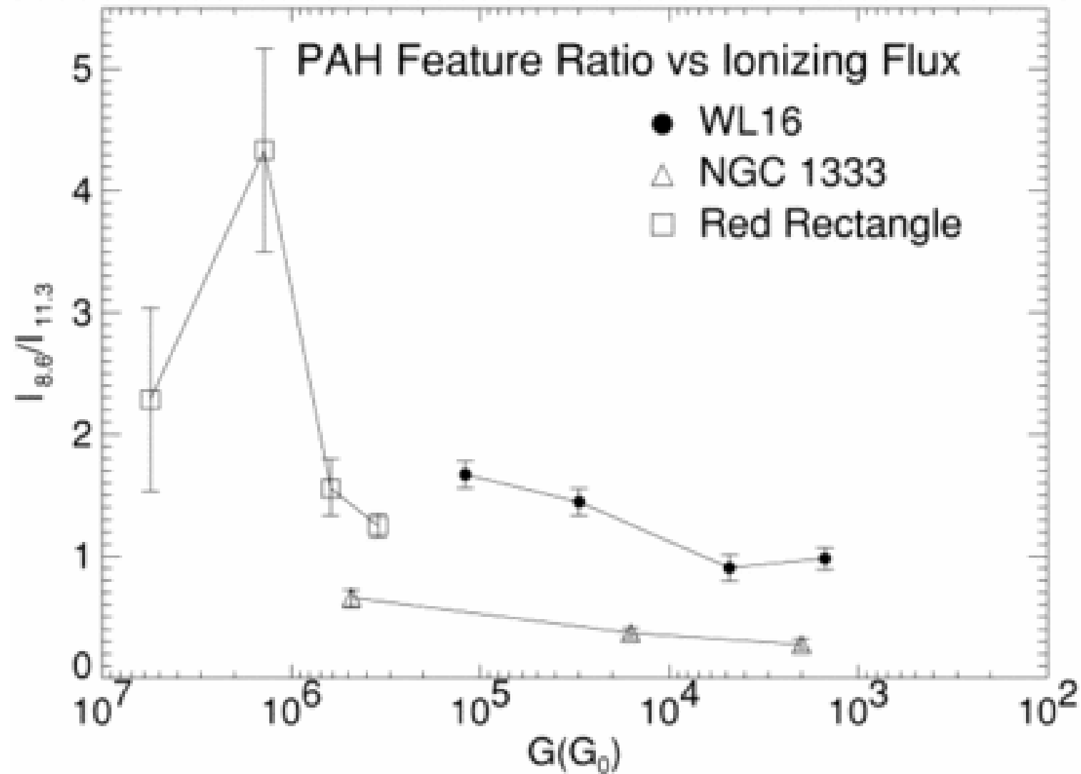
Fig. 5. from MidInfrared Emission Features in WL 16 DeVito & Hayward 1998 ApJL 504 L43 doi:10.1086/311565 https://dx.doi.org/10.1086/311565 © 1998. The American Astronomical Society. All rights reserved. Printed in U.S.A.
