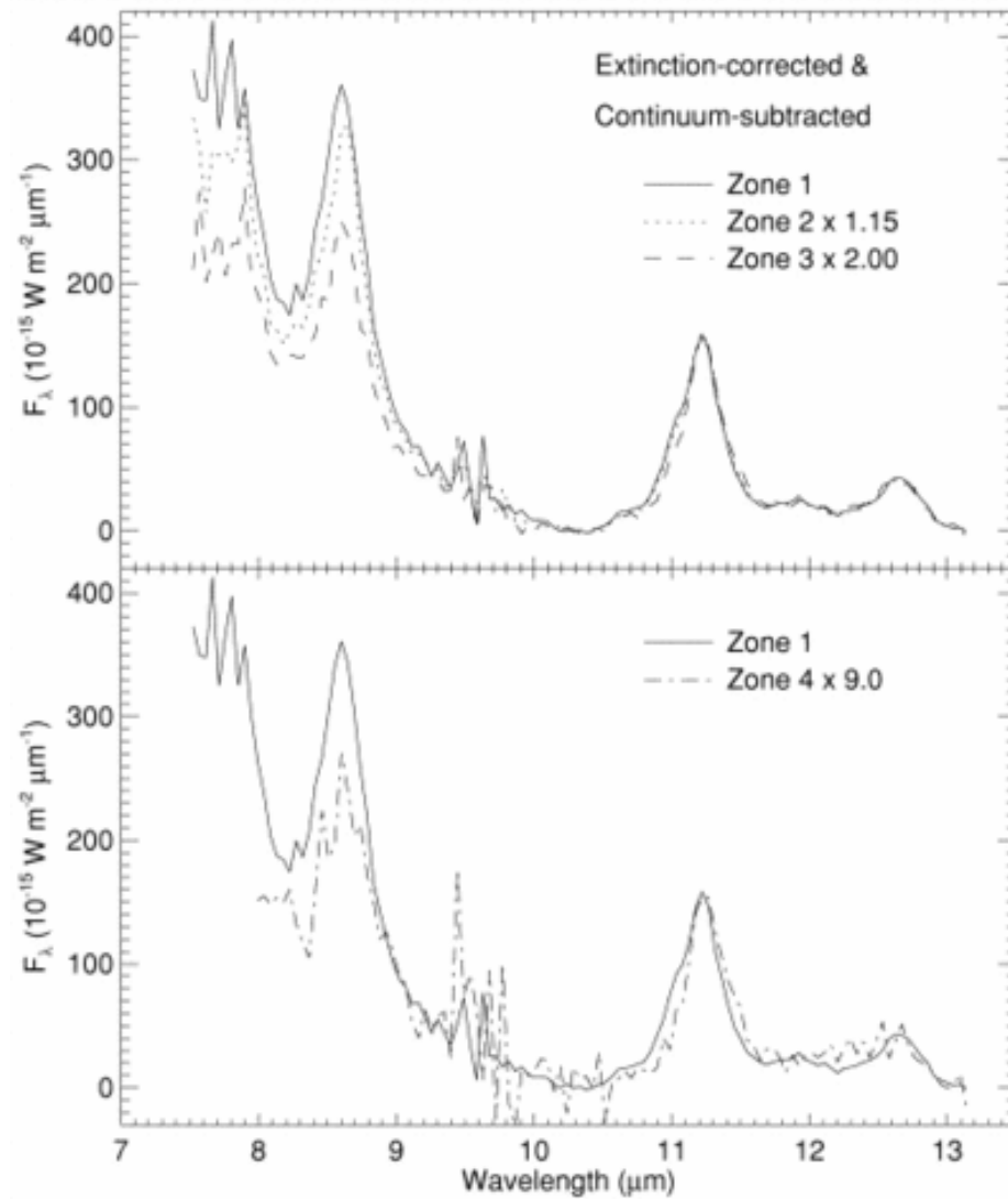
Fig. 3. from MidInfrared Emission Features in WL 16 DeVito & Hayward 1998 ApJL 504 L43 doi:10.1086/311565 https://dx.doi.org/10.1086/311565 © 1998. The American Astronomical Society. All rights reserved. Printed in U.S.A.
