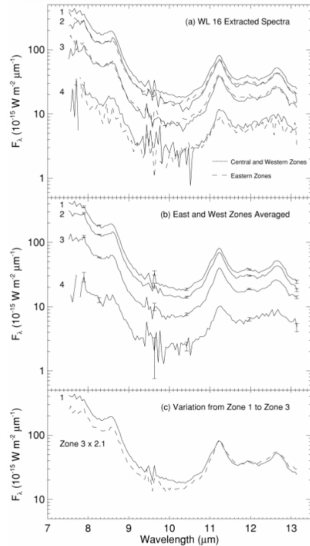
Fig. 2. from MidInfrared Emission Features in WL 16 DeVito & Hayward 1998 ApJL 504 L43 doi:10.1086/311565 https://dx.doi.org/10.1086/311565 © 1998. The American Astronomical Society. All rights reserved. Printed in U.S.A.
