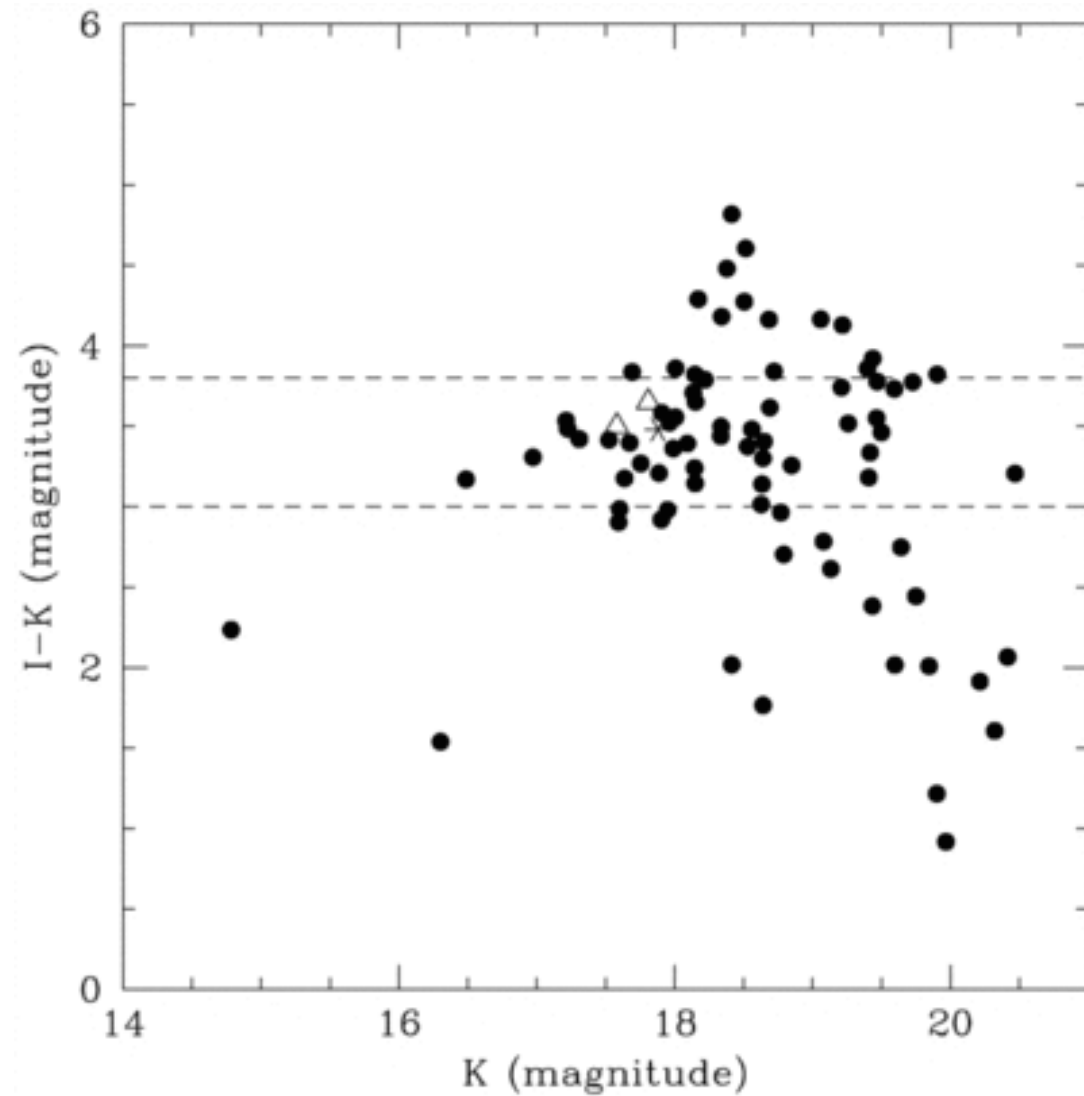
Fig. 3. from HighResolution Optical and NearInfrared Imaging of the Quadruple Quasar RX J0911.4+0551 Burud et al. 1998 ApJL 501 L5 doi:10.1086/311450 https://dx.doi.org/10.1086/311450 © 1998. The American Astronomical Society. All rights reserved. Printed in U.S.A.
